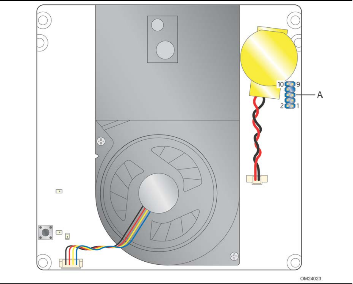
Figure 11. Header (Top)
