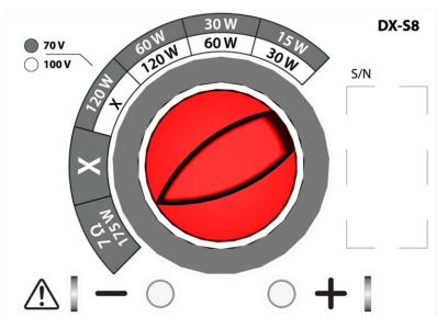
Tap Switch / Input Panel
