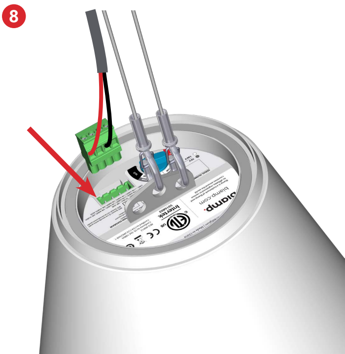
Install euroblock
