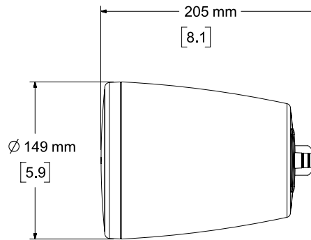
Right View DIMENSIONS APPLY TO BOTH SIDES
