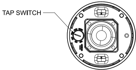
Front View GRILLE REMOVED FOR CLARITY
