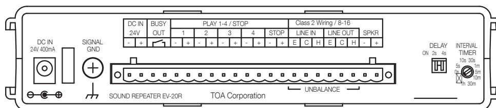
Rear View
