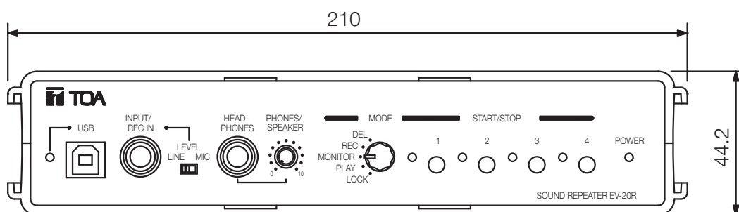
Front View
