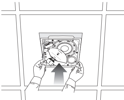
Fig. 1. Install loudspeaker.
