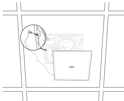
Fig. 2. Insert safety lanyard pin.
