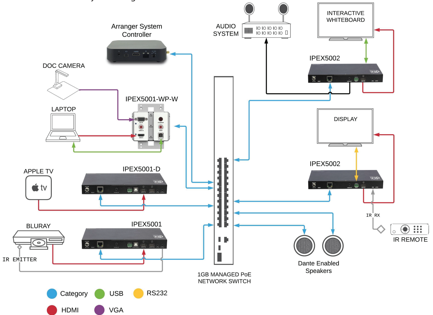
IPEX5000 Basic System Diagram
