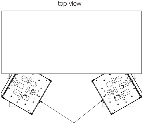
C5D-SRSR12 shown rotated 60° in both directions
