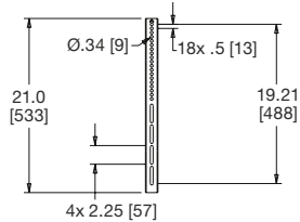
display mount bracket hole pattern
