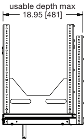
side view closed position
