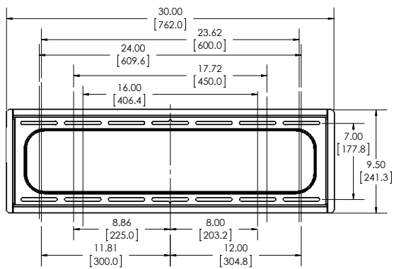
WALL PLATE
